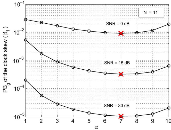
Fig. 2. Performance bound PB_g(\beta_1) of the estimated clock skew \hat{\beta}_1 using the generalized MLLE with different \alpha 's. The "x" indicates the value of \alpha calculated by (32), i.e., \alpha^* = 2k + \lceil j/2 \rceil , where k and j are related to N by N = 3k + j , with k \in \{0, 1, 2, 3, \dots\} and j \in \{0, 1, 2\} .
