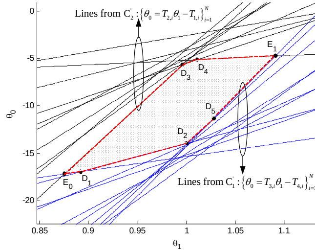
Fig. 2. Feasible region defined by \mathcal{C}'_1 and \mathcal{C}'_2 with N = 10 .
