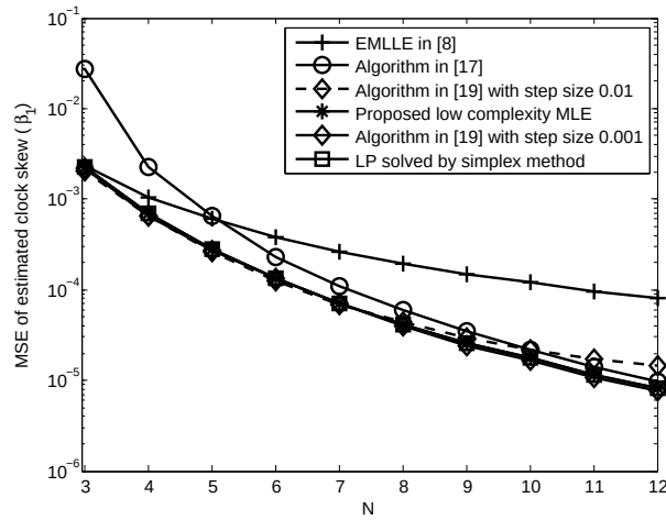
Fig. 5. MSE of estimated clock skew \hat{\beta}_1 with respect to the number of rounds of message exchange N .
