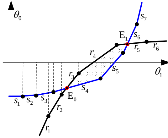
Fig. 3. Example of a feasible region defined by intersection of \{s_p\}_{p=1}^P and \{r_q\}_{q=1}^Q .
