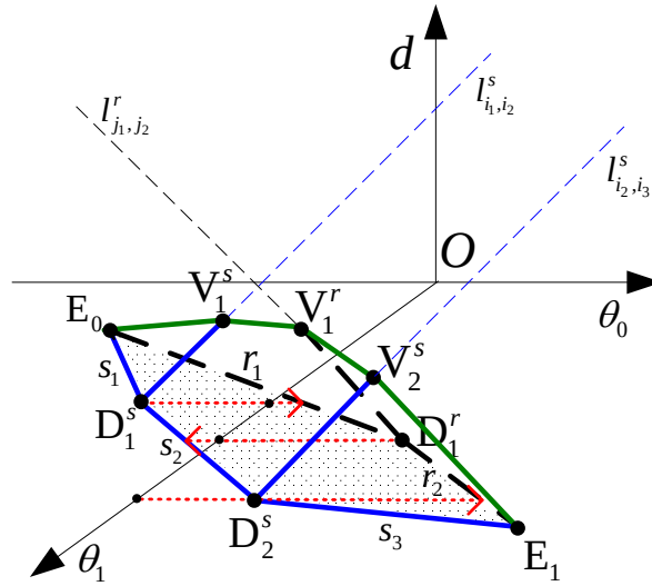
Fig. 4. Example of the domain S ; Vertices defined by C_1' and C_2' : \{E_0, D_1^s, D_2^s, D_1^r, E_1\} and Vertices defined by C_1'' and C_2'' : \{V_1^s, V_2^s, V_1^r\} .
