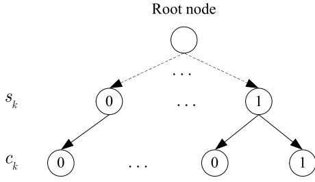
Fig. 2. Search tree of the MBB method.
