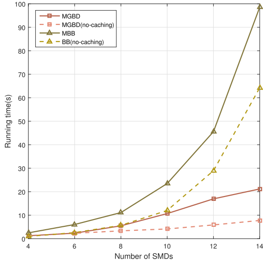
Fig. 5. Running time of MBB and MGBD.
