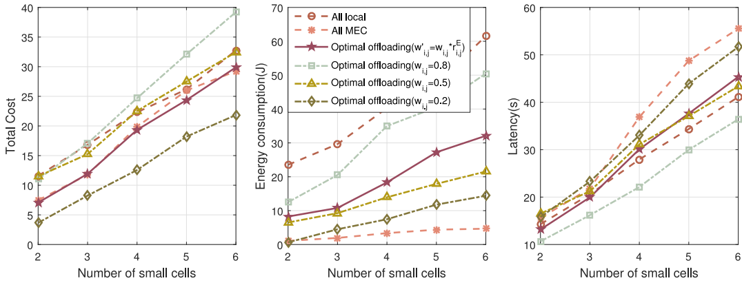
Fig. 5. Tradeoff between energy consumption of SMDs and execution latency of their tasks under different number of small cells.
