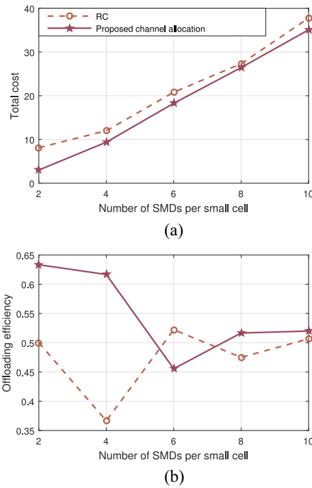
Fig. 8. Impact of channel allocation on the total cost and offloading efficiency. Impact of channel allocation on (a) total cost and (b) offloading efficiency.
