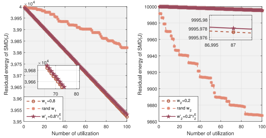
Fig. 4. Impact of the weightings on the residual energy of SMDs.
