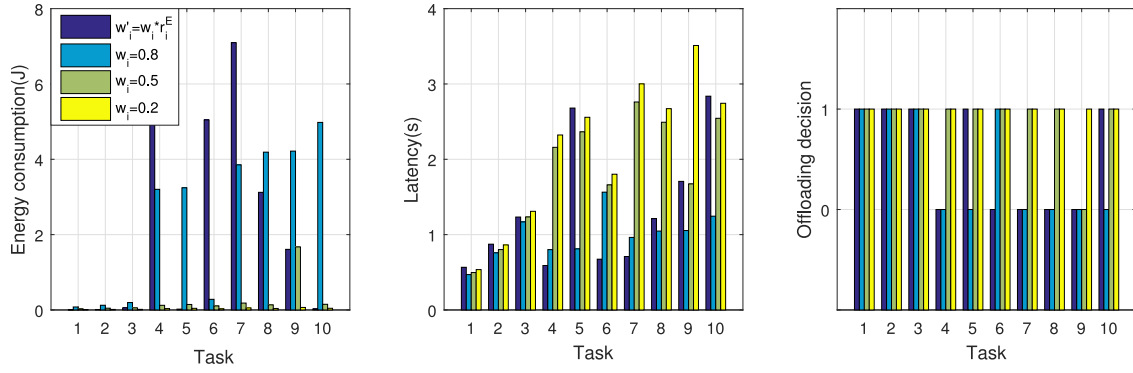
Fig. 3. Compact of weightings on energy consumption, latency, and the offloading decision.
