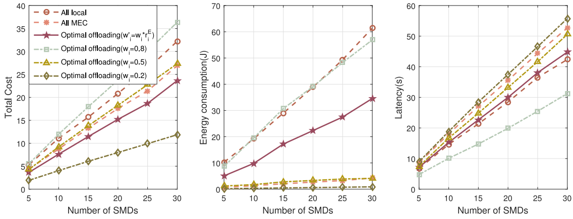
Fig. 2. Tradeoff between energy consumption of SMDs and execution latency of their tasks under different number of SMDs.
