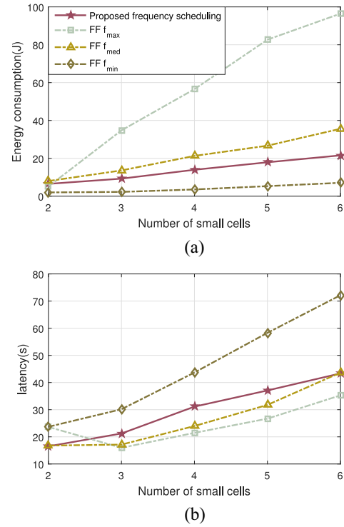
Fig. 7. Impact of the computation CPU-cycle frequency of SMDs on the energy consumption and execution latency under different number of small cells. Impact of the computation CPU-cycle frequency of SMDs on (a) energy consumption and (b) execution latency.
