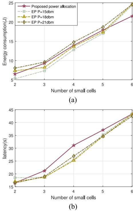
Fig. 6. Impact of the transmission power of SMDs on the energy consumption and execution latency under different number of small cells. Impact of the transmission power of SMDs on (a) energy consumption and (b) execution latency.
